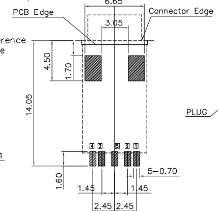
RECOMMENDED P.C.B LAYOUT TOLERANCE : ±0.05(TOP VIEW)
