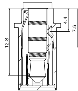
SEC: A-A IMAGE OF PLUG MATCH WITH CONTACT POINT
