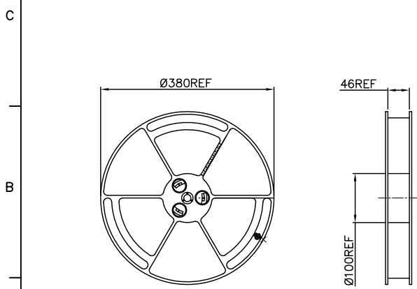
REEL FOR CARRIER TAPE
