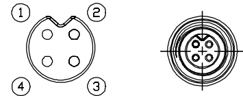
Front View Pin Assignment
