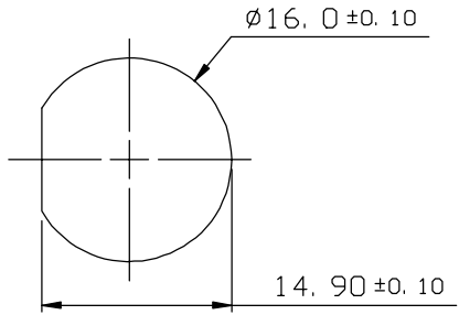
PANEL CUT OUT DIMENSION
