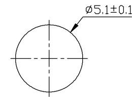
Recommend Panel Cut-Out
