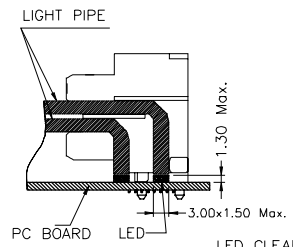
LED CLEARANCE REQUIREMENTS
