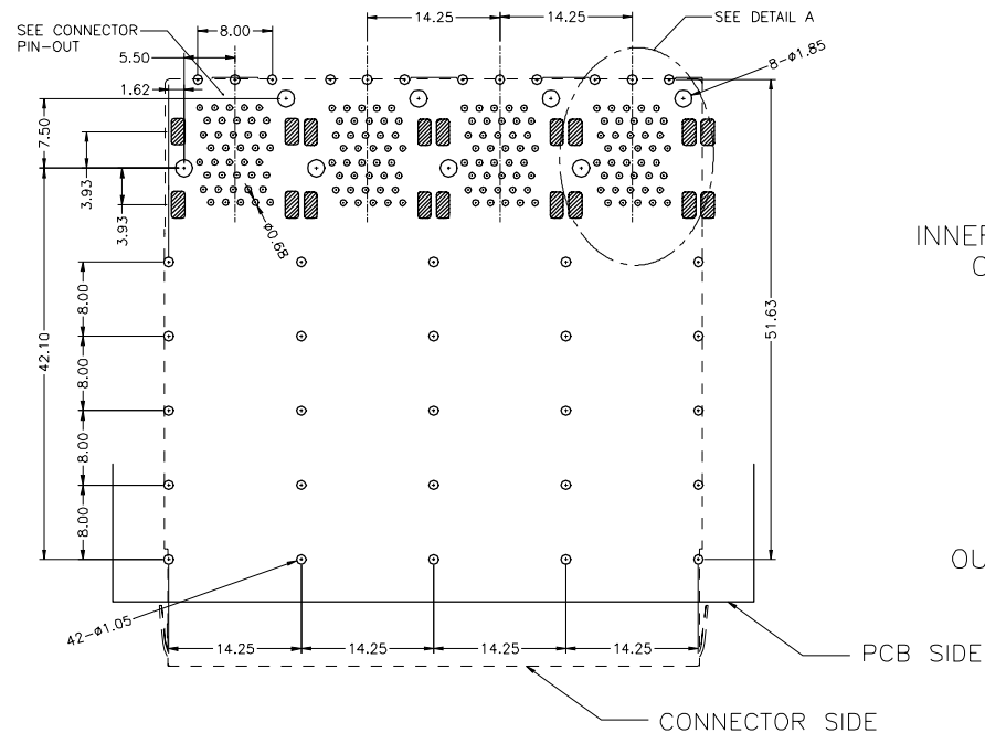
P.C.B. LAYOUT TOP VIEW \pm 0.05
