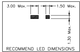
LED CLEARANCE REQUIREMENTS
