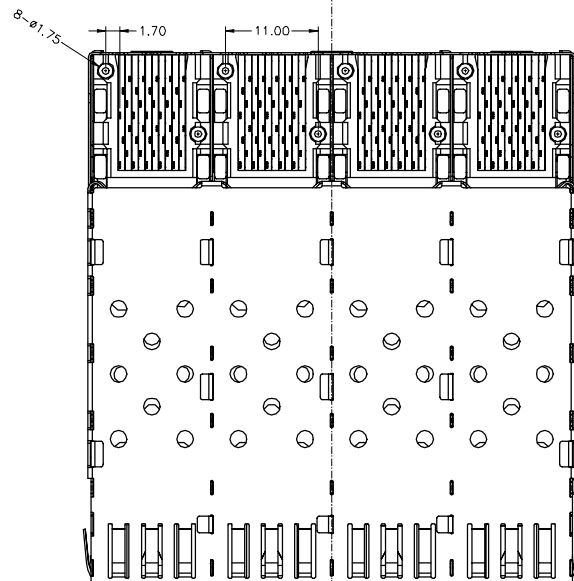
P.C.B. LAYOUT TOP VIEW \pm 0.05
