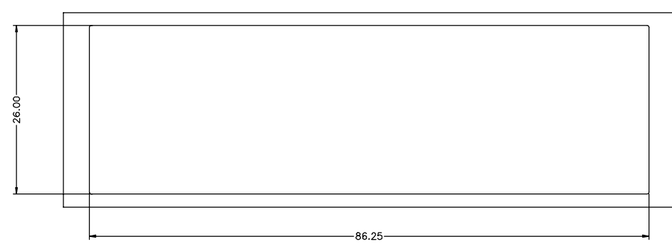
BEZEL CUT-OUT CENTER SPACING DETAIL BEZEL THICKNESS:0.8-2.6
